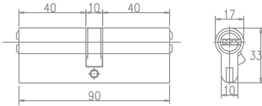
FW60.713 Barel Cylinders
